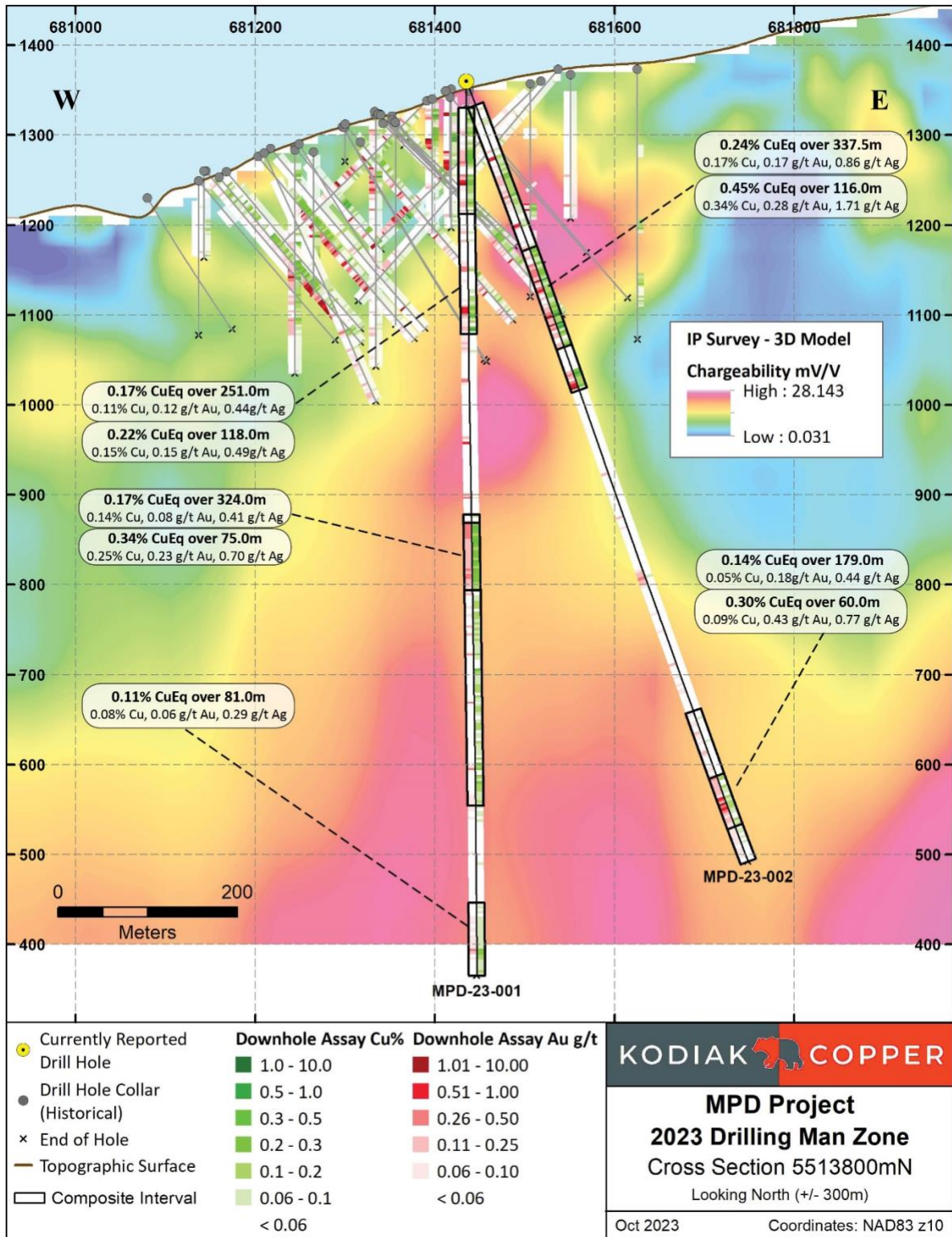
Figure 3: Man Zone east-west long section at 5513800mN (looking north). Background is colour contoured 3D IP Chargeability. See Table 1 for results from new holes MPD-23-001 and MPD-23-002
